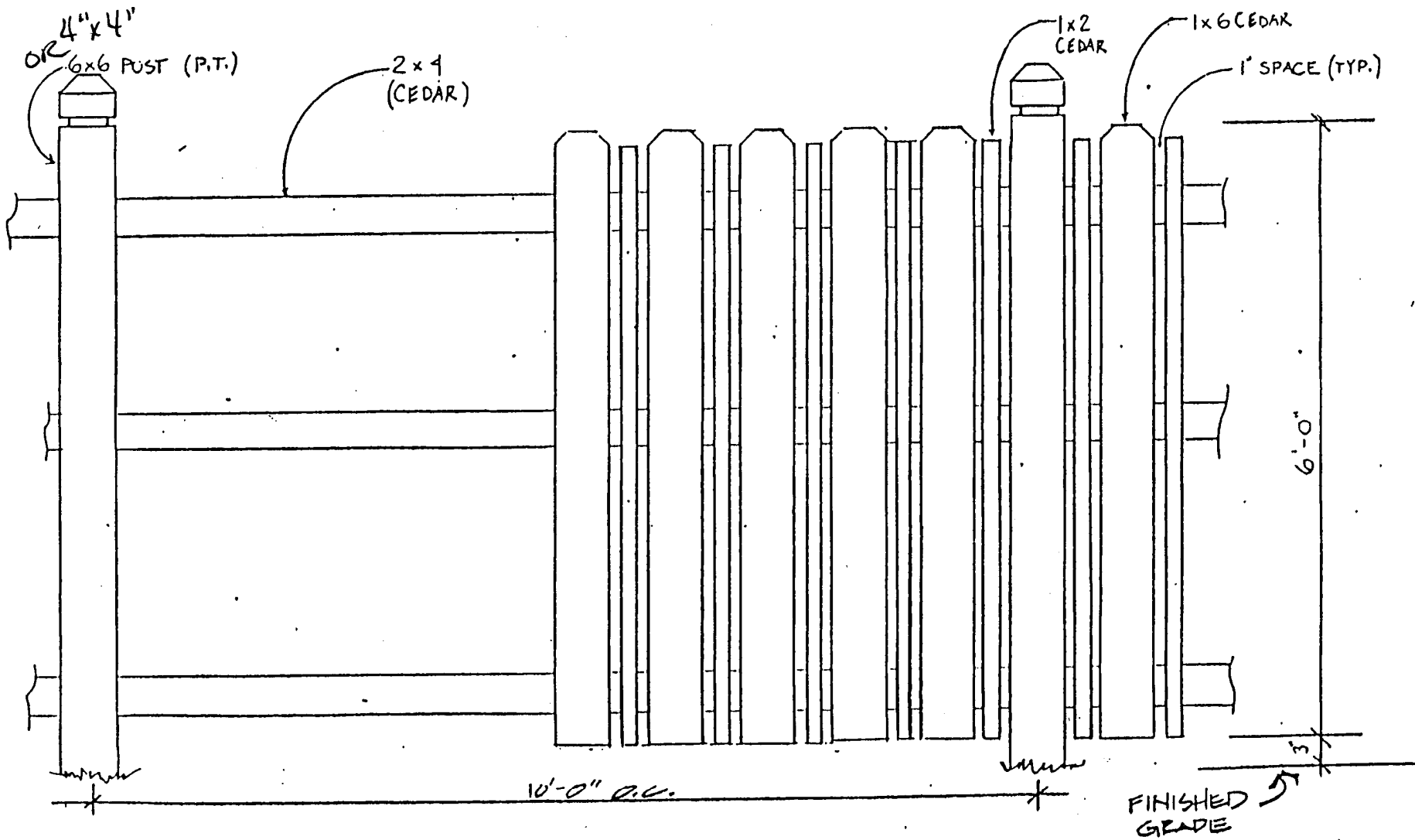
FENCE DETAIL 'D' NOT TO SCALE
